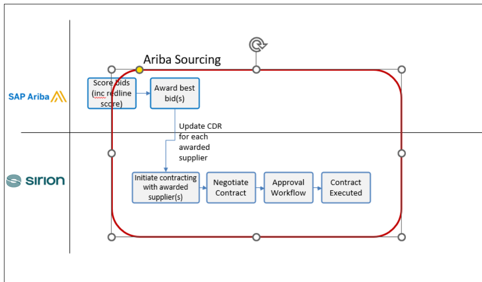
Figure 1: Integration Workflow
